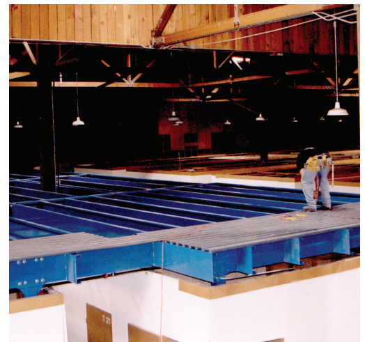
ResinDek® MD panels installed in 2003
