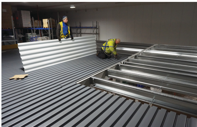
Installation of Corrugated B Deck in Client's Cold Storage Warehouse
